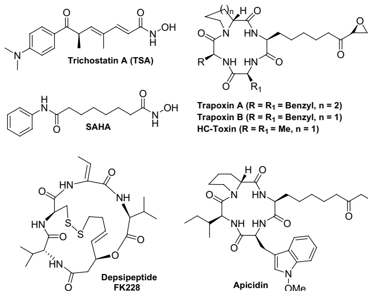
Figure 1. Structure of some known HDAC inhibitors.
