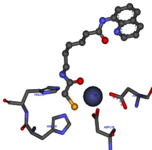
Figure 3. Compound 10b docked into the binding site of HDAC1.
