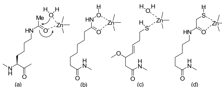
Figure 2. Possible mode of interaction of the zinc ion of HDAC with (a) acetylated lysine moiety of histone, (b) hydroxamate group of an HDAC inhibitor, (c) thiol group from FK228 + DTT, (d) our designed mercaptoacetamide-based inhibitors.
